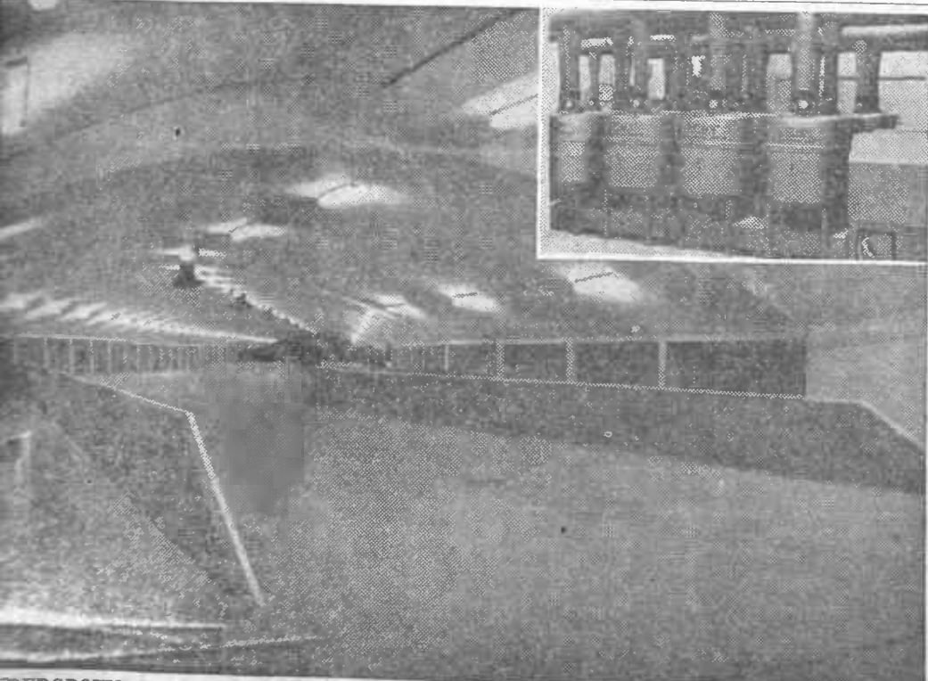
UNDERGROUND PARKING garage in Stockholm, Sweden, showing two levels in this vast dual-purpose civil defense shelter which can accommodate 1000 persons. The garage, a key unit in the large civil defense program in the world today, is equipped with triple electric doors at the entrance ramp to wall out blast pressures, electric generators, and a special air filter system, (inset) to eliminate poison gas, germs and radioactive dust. (Swedish Civil Defense Photo)
